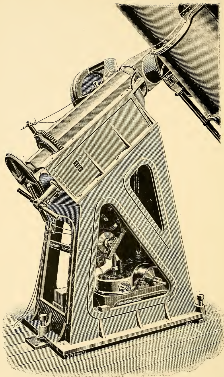
THE DRIVING CLOCK OF THE ASTROGRAPHIC TELESCOPE.
