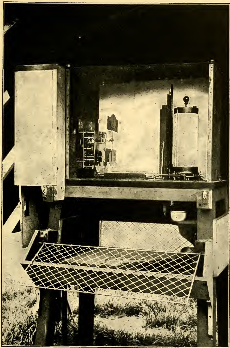
THE SELF-REGISTERING THERMOMETERS.
