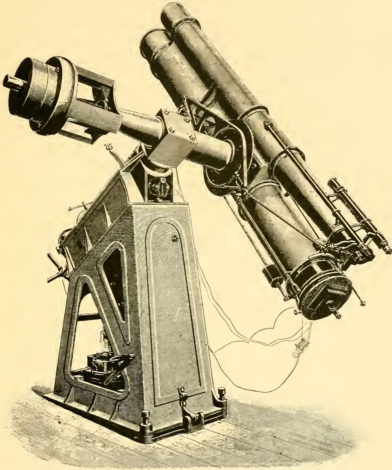
THE ASTROGRAPHIC TELESCOPE.
